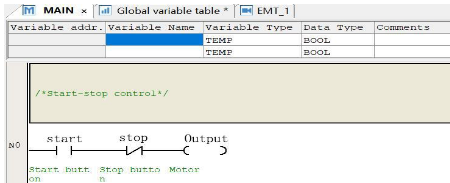
Figure 4-10 Ladder program when component comment is displayed
