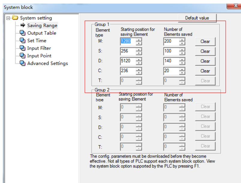
Figure 2-3 Configuration save element address range
