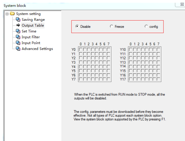
Figure 2-4 set output table
