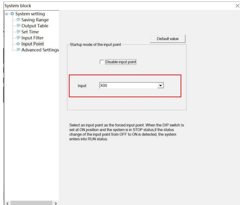
Figure 2-7 set input point
