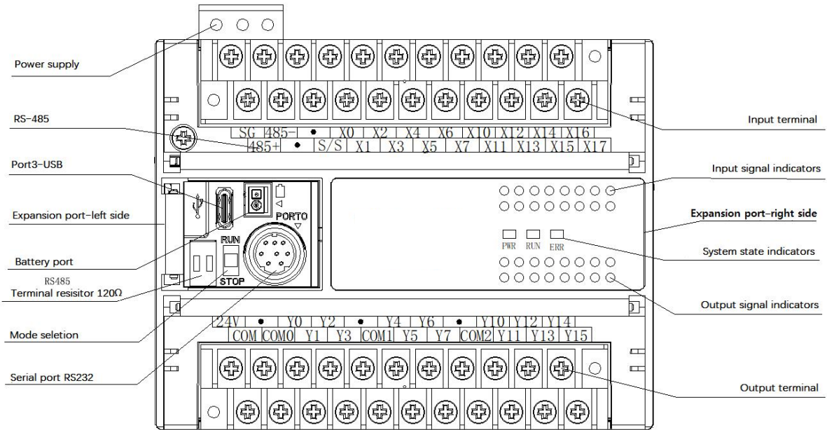
Figure 1-1 VIC-B series main module outline structure
