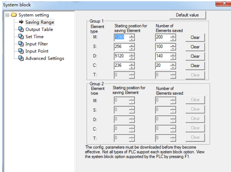
Figure 2-2 Set save range
