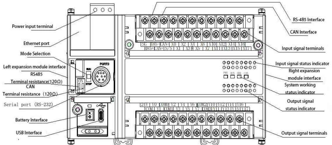
Figure 1-2 VIC-S series main module outline structure
