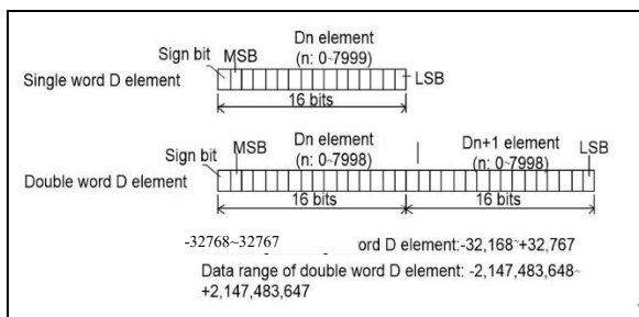
Figure 3-5 D or R element
