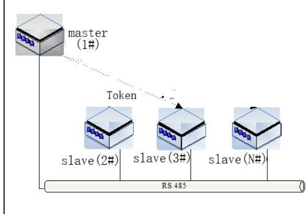
Figure 10-4 The master issues a token to the 3# slave
