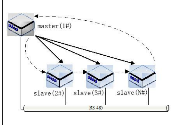
Figure 10-6 Token issuance and flow sequence
